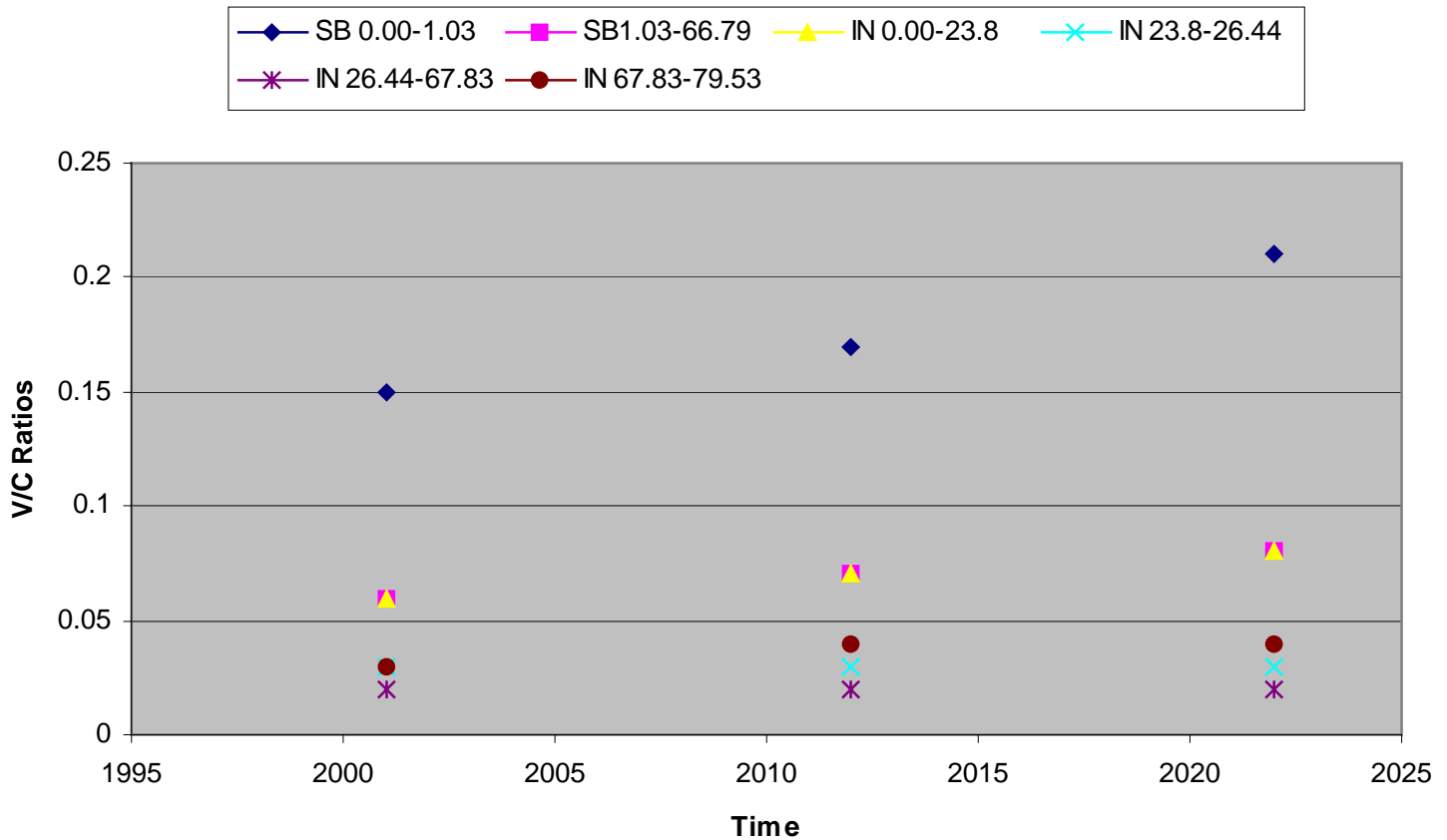
SR 127 Volume to Capacity Ratios as Function of Time for Six Different Segments
